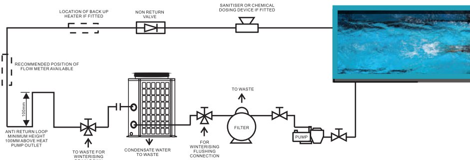
Recommended plumbing diagram
