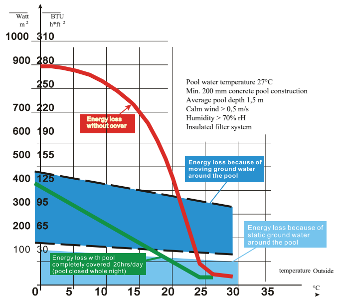
Energy Loss Graph
